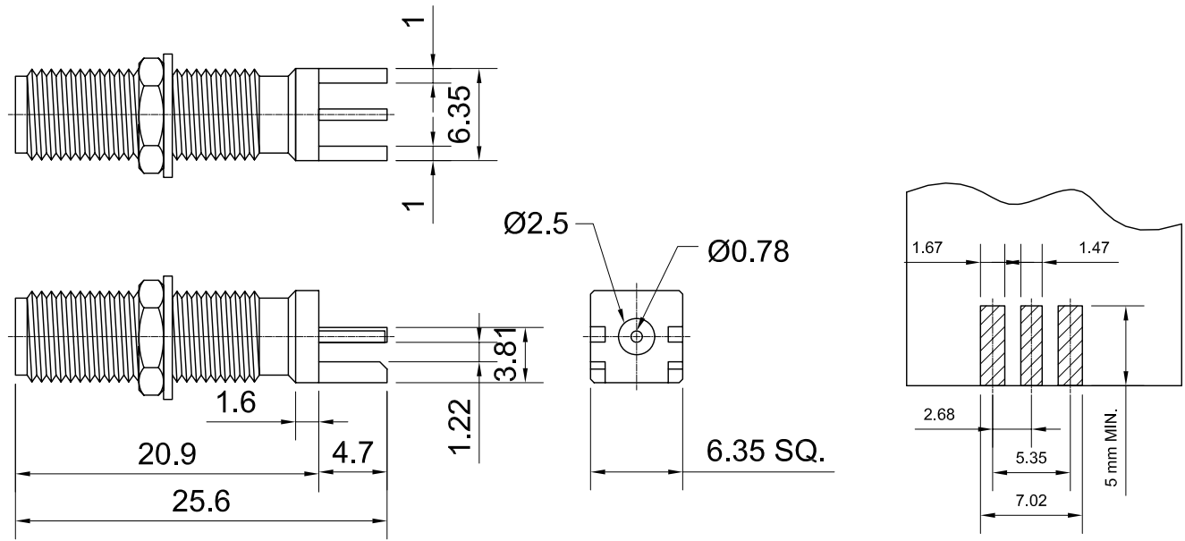
LANDING PAD DIMENSIONS
